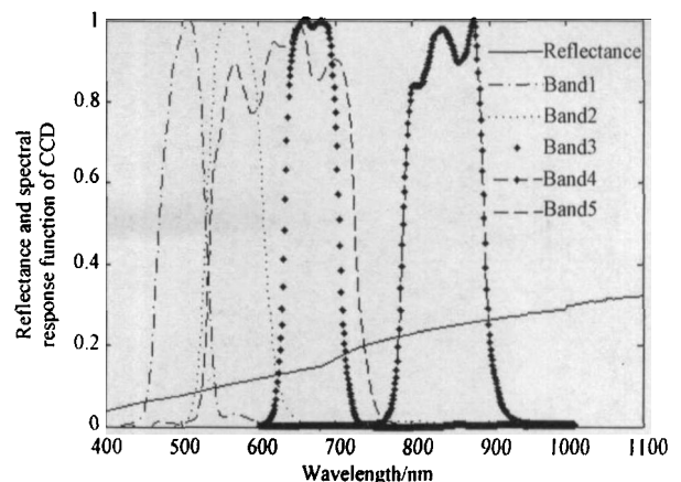
Fig. 3 Surface reflectance results of the test site and spectral response function of CCD
