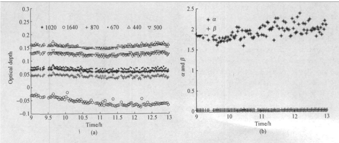
Fig. 4 Optical properties of atmospheric aerosol on Oct 12, 2007 (a) Aerosol optical depth changed with time; (b) Parameters
